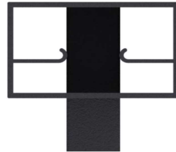
Top/Bottom Rail Profile (shown w/ baluster)
